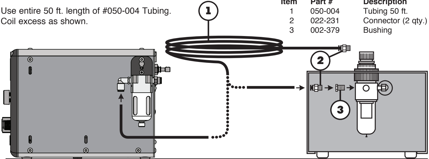
CONNECTION FOR GRAVERMACH or GRAVERMAX SC
